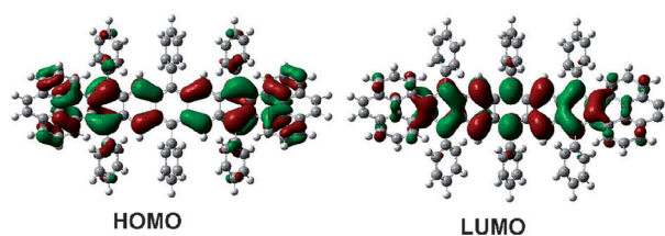
Figure 4. Wave function plot for the HOMO and LUMO of 2 .
