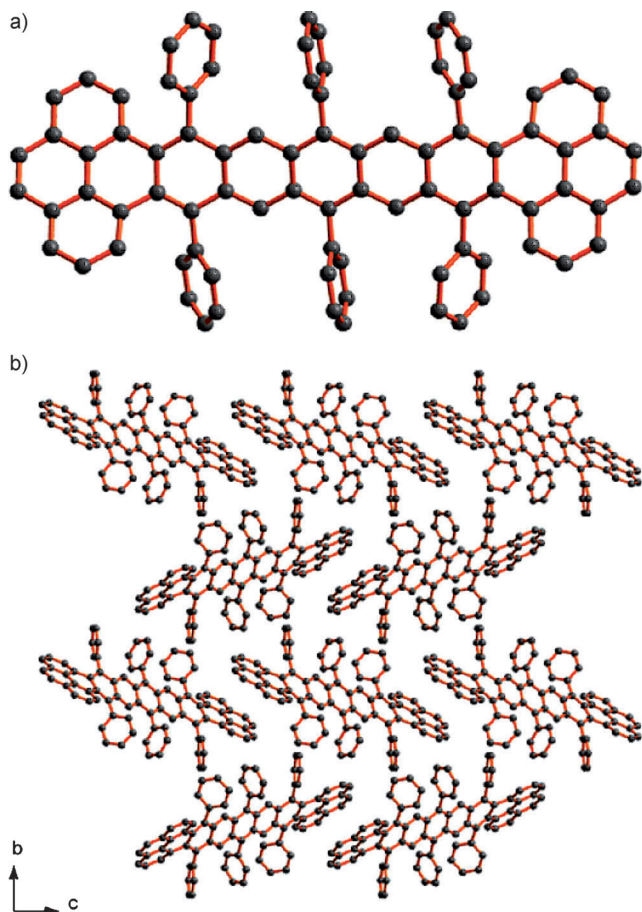
Figure 2. Single crystal analysis of 1 . a) One molecule unit. b) Molecular packing.
