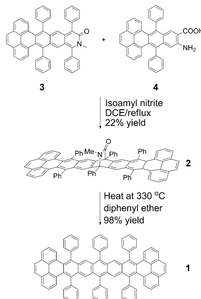
Scheme 2. Synthesis of 6,8,10,17,19,21-hexaphenyl-1,22,4,5,11,12,15,16-tetrabenzononatwistacene ( 1 ). DCE = 1,2-dichloroethane.
