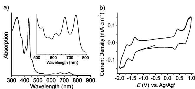
Figure 3. a) The UV-Vis absorption spectra of 1 in CH 2 Cl 2 . The inset shows the magnified spectrum. b) Cyclic voltammogram of 2 in 1,2-dichlorobenzene using tetrabutylammonium perchlorate as an electrolyte.
