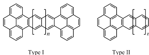
Figure 1. Twistacene structures.
